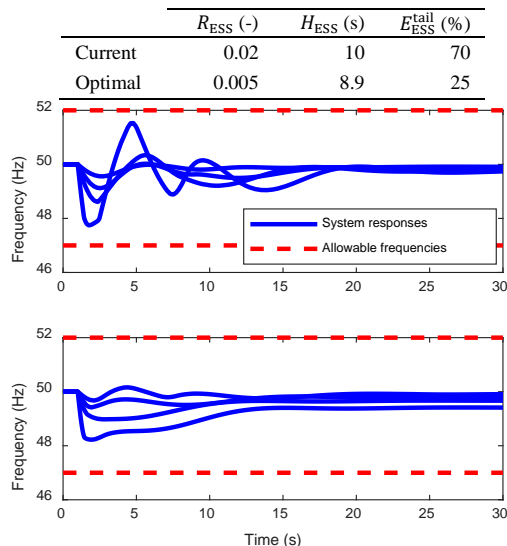
Figure 7. Frequency response of the Spanish island system for the four representative contingencies. Red-dashed horizontal lines indicate \omega^{\min} and \omega^{\max} . Top panel: Current UFLS and UC. Bottom panel: Optimal UFLS and UC
