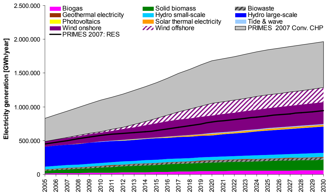
Figure 9: GreenNet BAU simulation results including projections until 2030 and conventional CHP updates for electricity generation on European level
